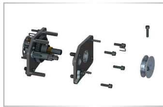
ACUdraw schematic.
